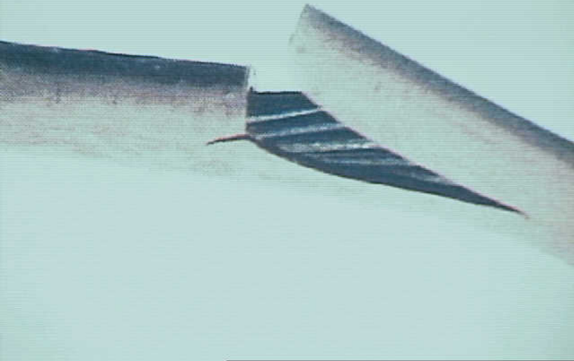
Systems 9 - Aging Aircraft Wire Testing - Photo 21. Cracking following 148 hours at 200 degree C and Bend Test.
