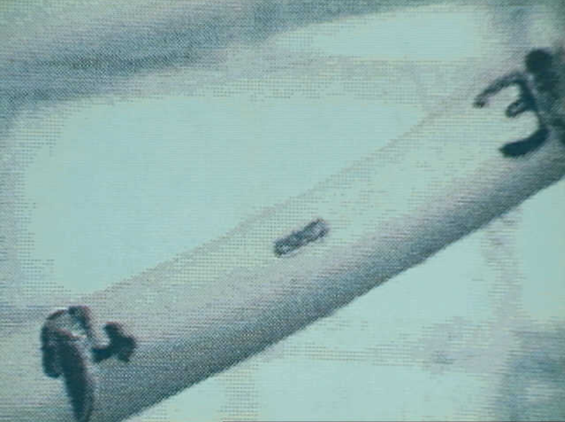
Systems 9 - Aging Aircraft Wire Testing - Photo 2. Cracks at Hot Stamp Marks
