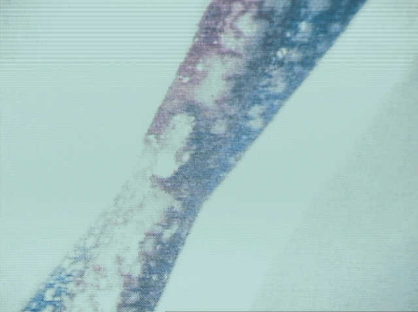
Systems 9 - Aging Aircraft Wire Testing - Photo 17. White Residue.
