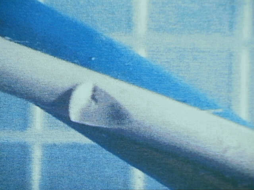
Systems 9 - Aging Aircraft Wire Testing - Photo 14. Gouges in Insulation.
