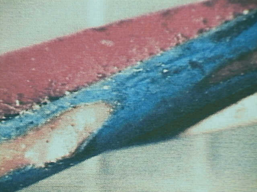
Systems 9 - Aging Aircraft Wire Testing - Photo 12. Chafing of Insulation.
