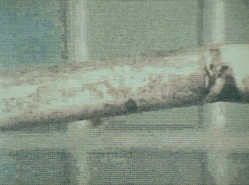
Systems 9 - Aging Aircraft Wire Testing - Photo 10. Gouge in Insulation.
