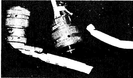
Photograph A3: White 747 Sample 1 Connectors
