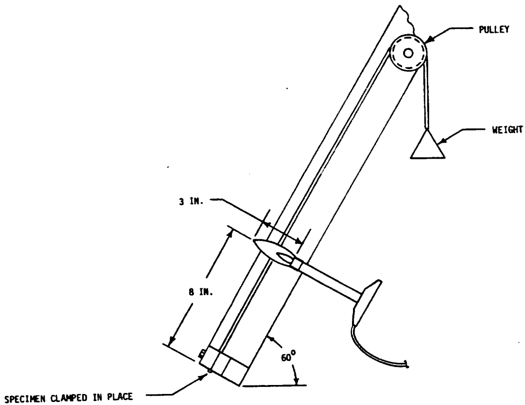
FLAMMABILITY TEST APPARATUS
