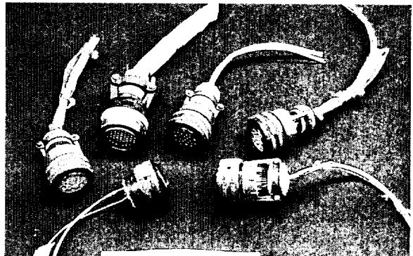
Photograph A6: European 747 Sample 1 Connectors
