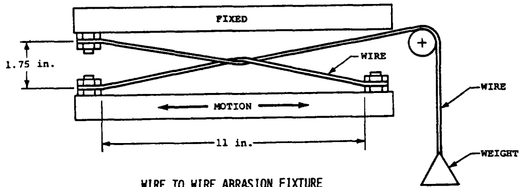
WIRE TO WIRE ABRASION FIXTURE
