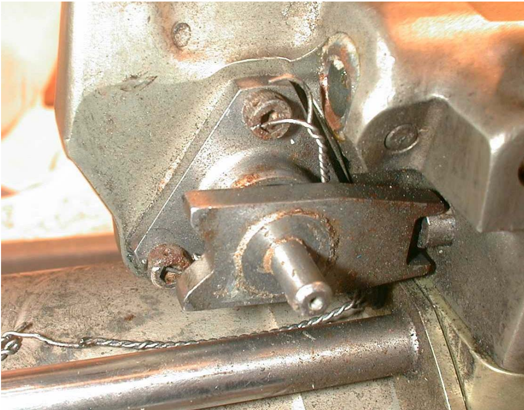
Figure 7. Test Finger in Extended Position.
