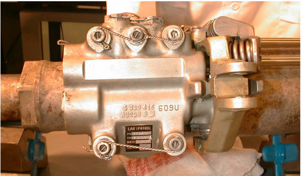
Figure 4. Control Valve Block and Input Lever Assembly.
