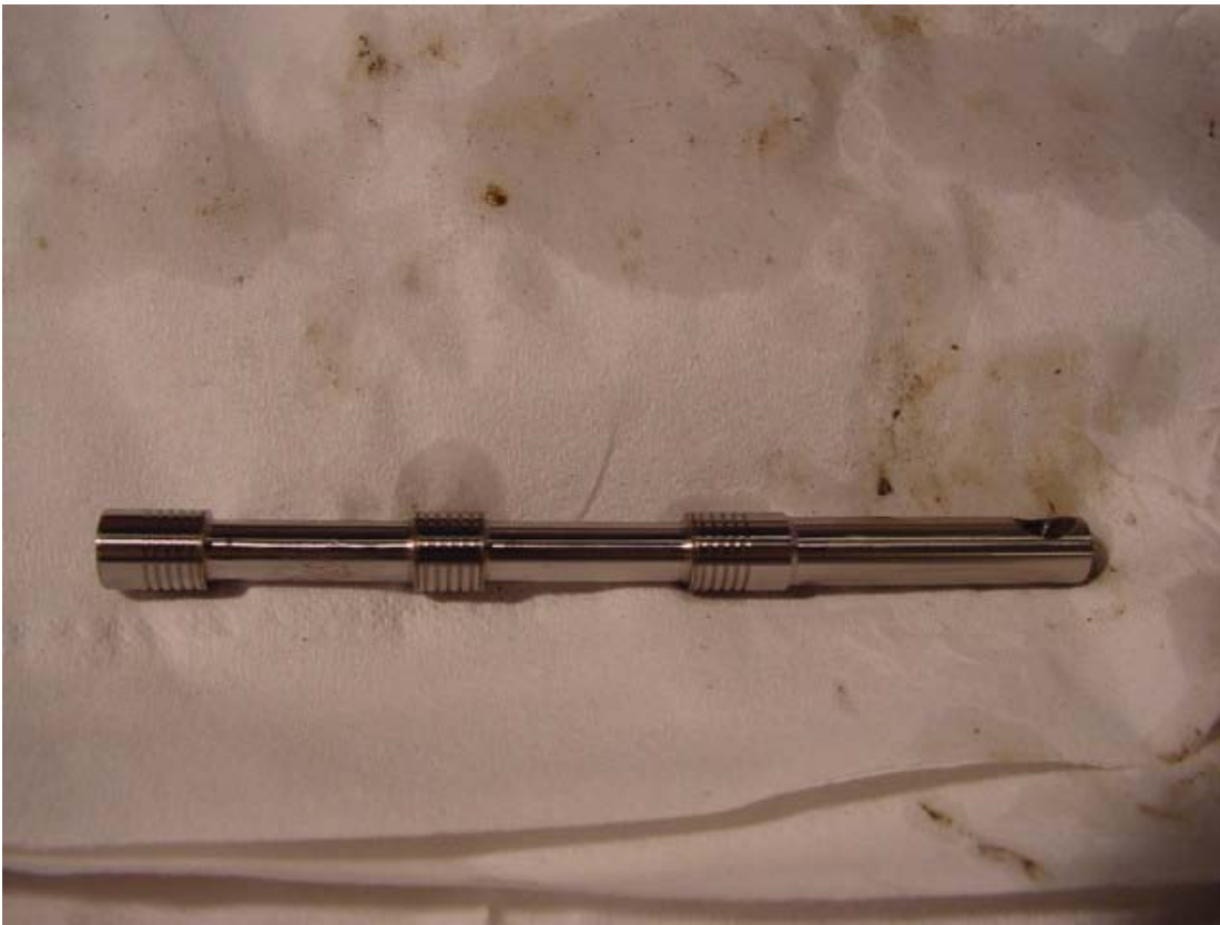
Figure 16. Main Control Valve Spool.
