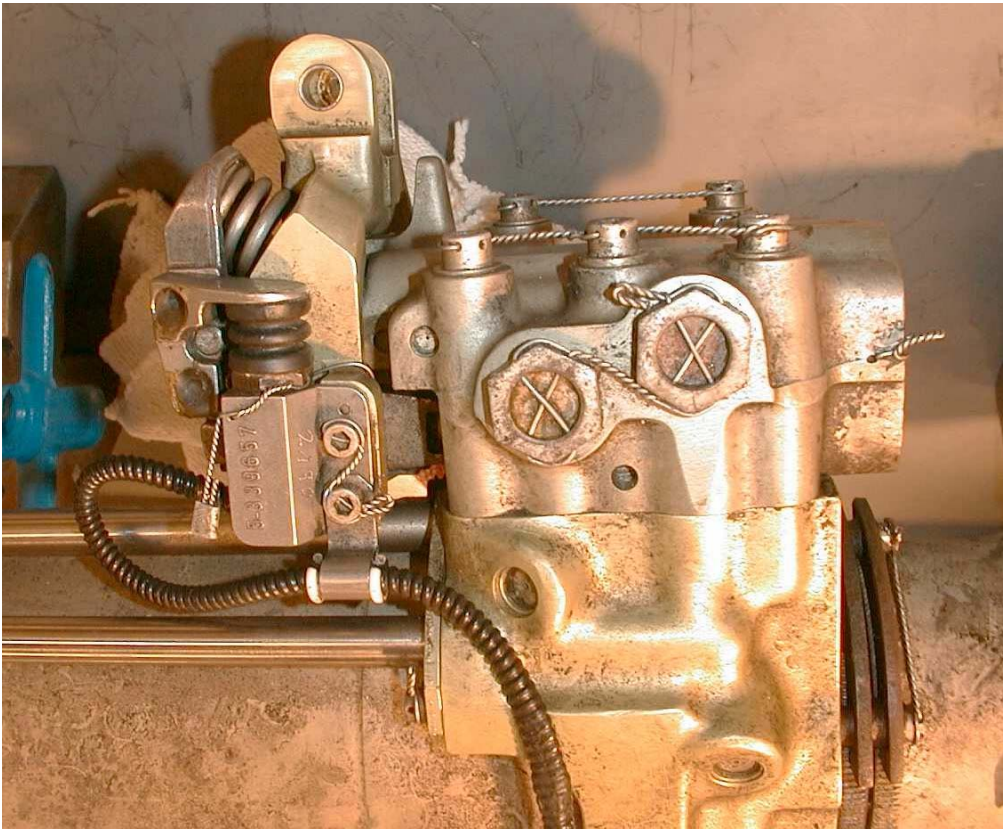
Figure 5. Control Valve Block and Input Lever Assembly.
