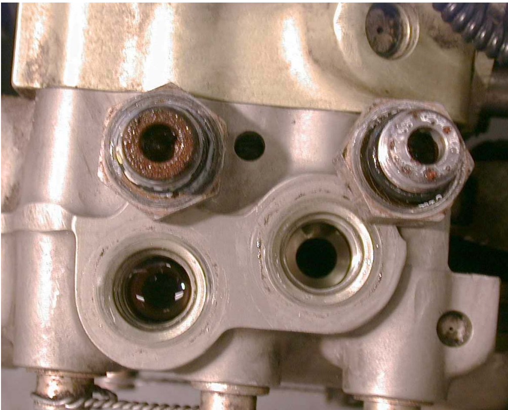
Figure 6. Hydraulic Ports Ca and Cb.
