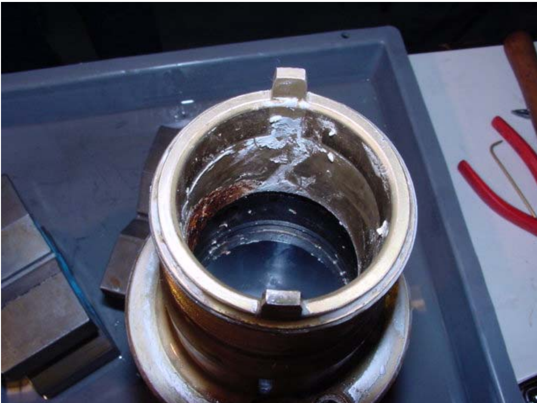
Figure 20. Fixed Rod End Retainer.
