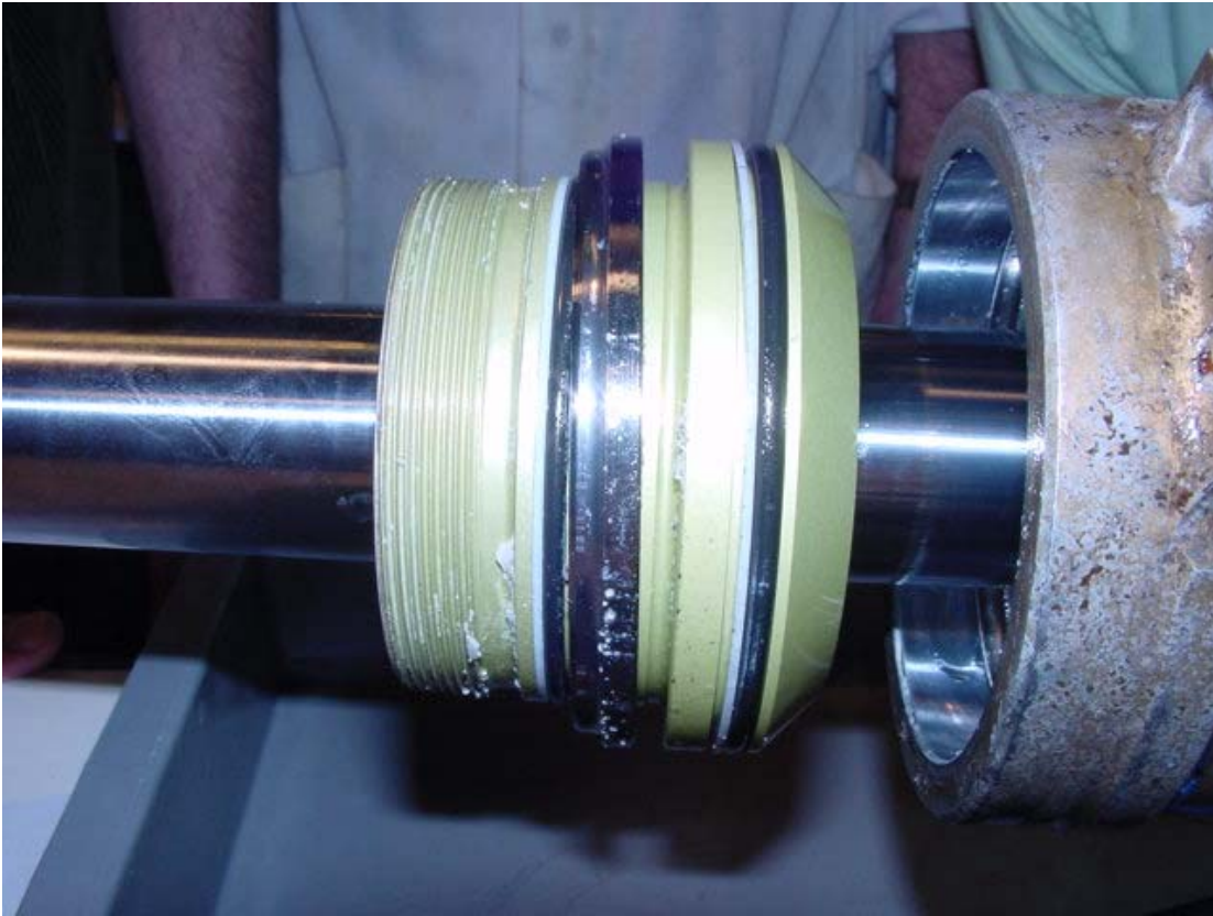
Figure 16. Piston End Bearing and Seal Assembly
