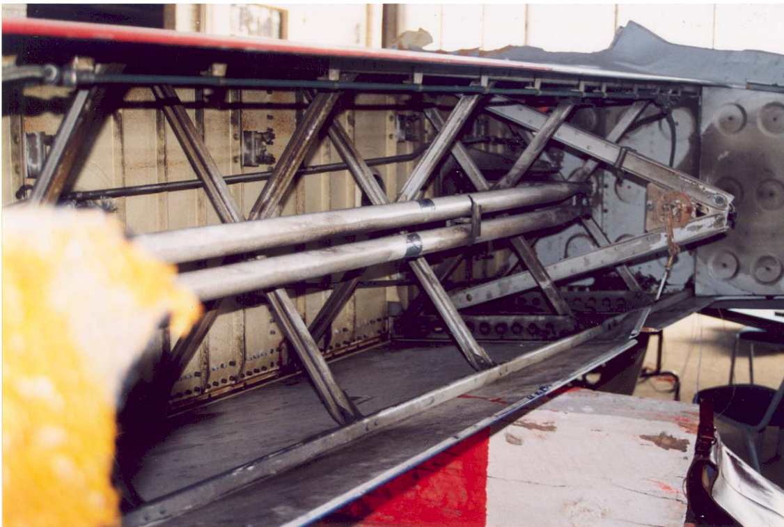
Figure 4. Pushrods Between Servos and Hinge 1.
