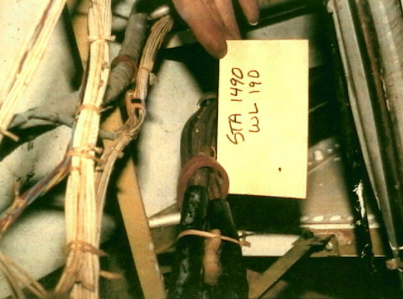
Systems 9 - 747-SL-30-048 - Fig. 32. Power feeders in good condition. Splices should be inspected for signs of over-heating.
