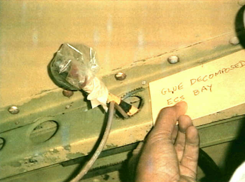
Systems 9 - 747-SL-20-048 - Fig. 9(a). In locations where wire bundles route through structure, caterpillar grommets or other protective material should be replaced when they fail.
