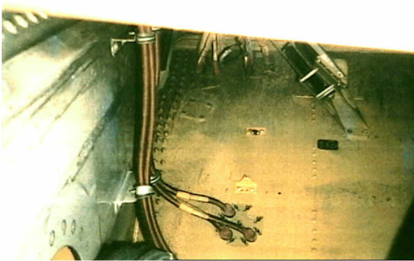
Systems 9 - 747-SL-20-048 - Fig. 8. A wing-body pressure seal penetration in good condition. Inspections should ensure the seals have not been compromised.
