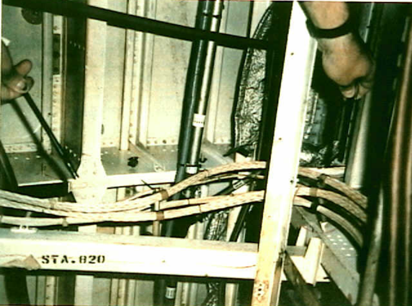
Systems 9 - 747-SL-20-048 - Fig. 7. Bent clamp bracket causing excess bundle length further down the bundle.
