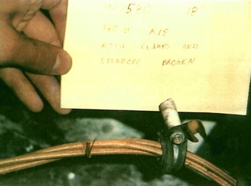
Systems 9 - 747-SL-20-048 - Fig. 6. Failed bundle clamps and standoff. Again, wire and adjacent clamps experience additional stresses.
