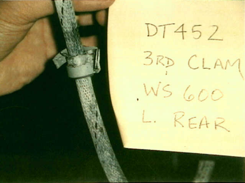
Systems 9 - 747-SL-20-048 - Fig. 5. Damaged cushion on a bundle clamp. Cushion can be damaged by mechanical forces or chemicals. Here no damage to the sleeving was observed.
