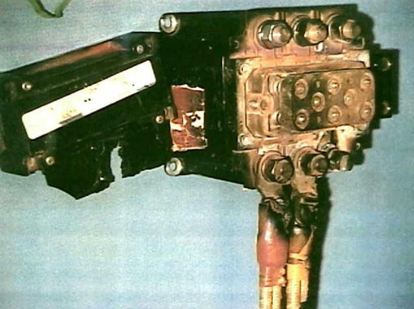
Systems 9 - 747-SL-20-048 - Fig. 37. Bus Tie Breaker overheated due to incorrect lug build-up.
