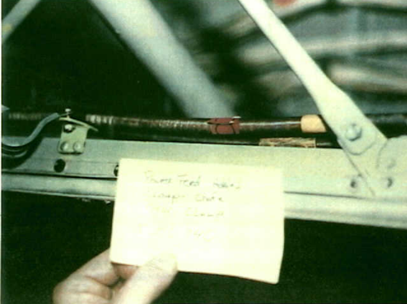
Systems 9 - 747-SL-20-048 - Fig. 35. Power feeders chafing at clamping points.
