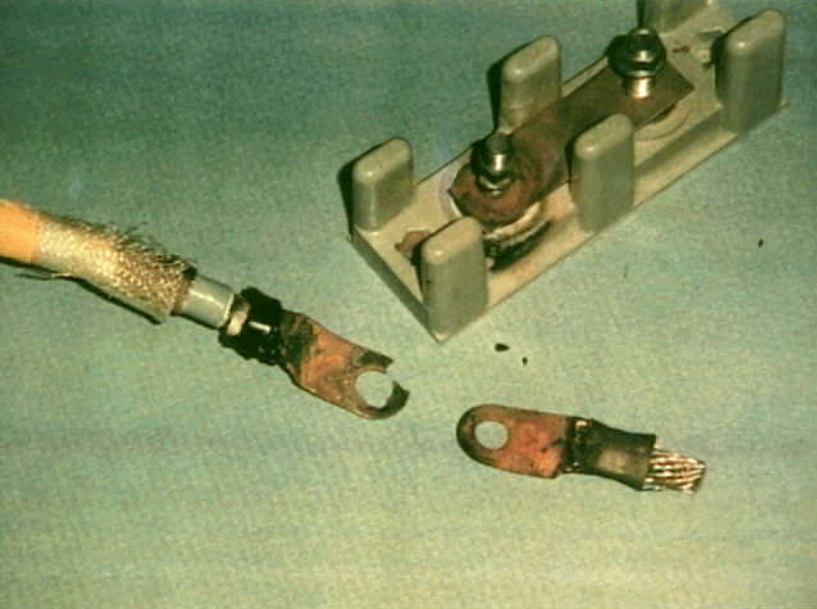
Systems 9 - 747-SL-20-048 - Fig. 34. High-current-carrying terminations with damage.
