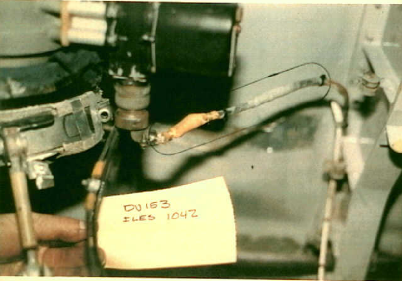
Systems 9 - 747-SL-20-048 - Fig. 30. Wire bundle to the leading edge power drive unit sleeved in service.
