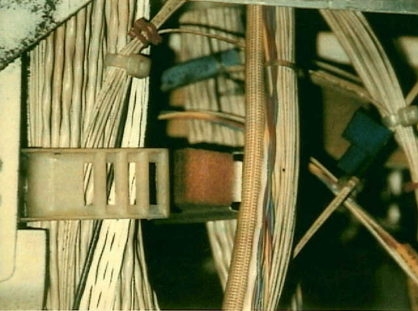
Systems 9 - 747-SL-20-048 - Fig. 3. Sprung open raceway clamp. This creates additional stress on wire and adjacent clamps. In this instance no wire damage was observed.
