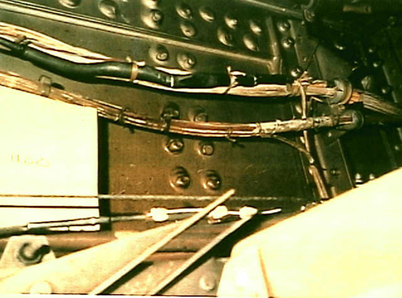
Systems 9 - 747-SL-20-048 - Fig. 27. Prior wire repairs. When examining wiring, inspect prior repairs carefully.
