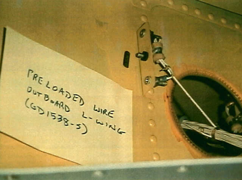
Systems 9 - 747-SL-20-048 - Fig. 26. Wires with a preload are susceptible to breakage at clamps and terminations. Tension on single conductors should be eliminated when possible.
