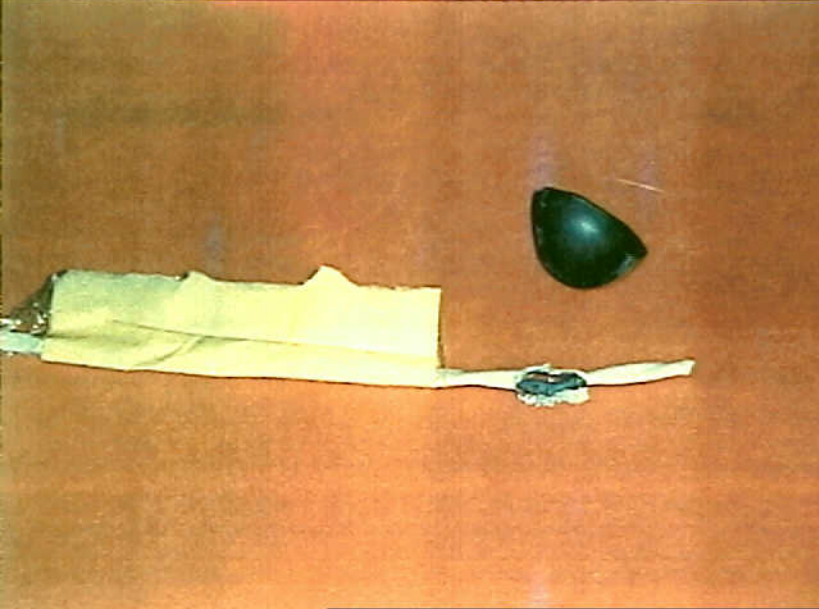
Systems 9 - 747-SL-20-048 - Fig. 25. Landing gear wire damaged by the debris thrown up by the tires. Here the damage was readily apparent.
