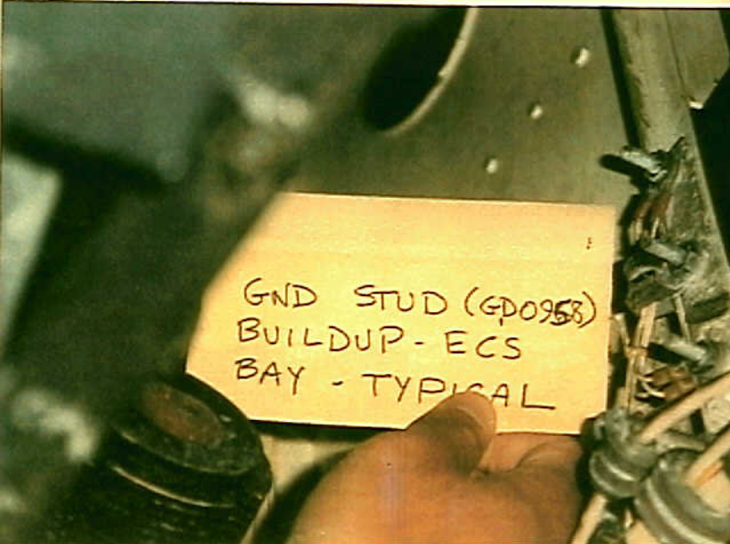
Systems 9 - 747-SL-20-048 - Fig. 24. If ground studs appear to exhibit corrosion, the ground resistance should be measured by a bonding meter to insure ground integrity.
