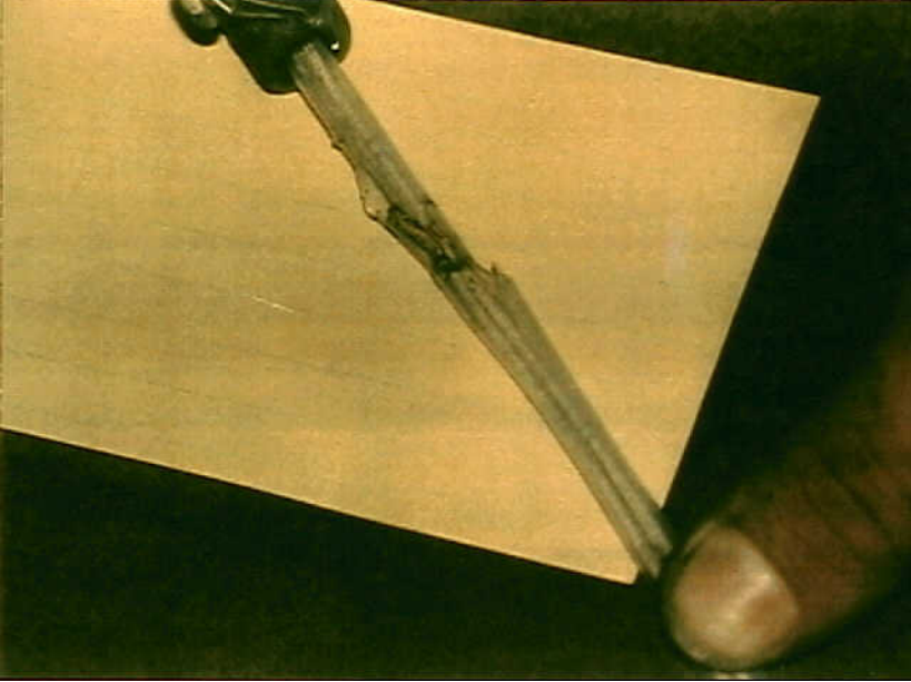
Systems 9 - 747-SL-20-048 - Fig. 23. Damage to Teflon sleeving due to lacing tape internal to the sleeving. Boeing does not recommend the use of lacing tape inside sleeving or conduits.
