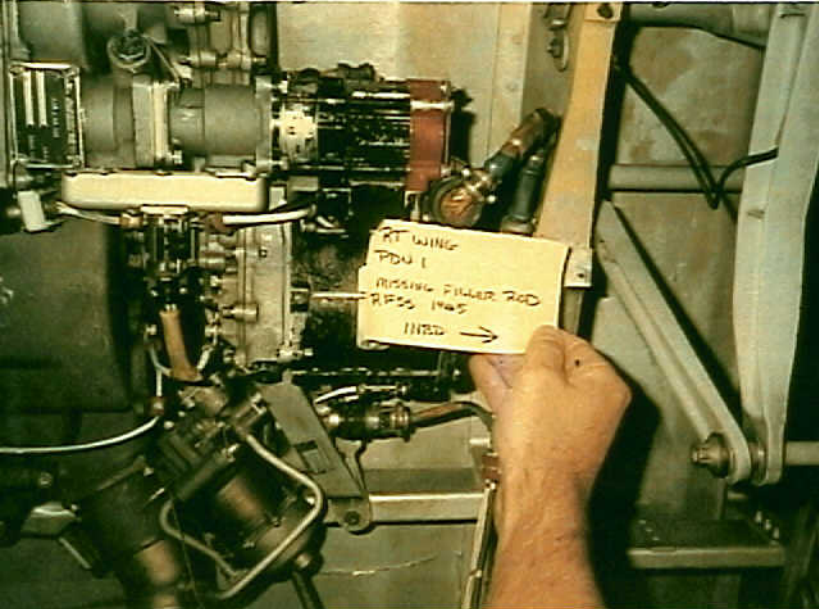
Systems 9 - 747-SL-20-048 - Fig. 22. Missing connector seal rods in unused contact cavities.
