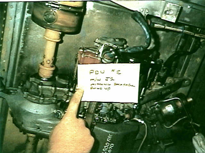
Systems 9 - 747-SL-20-048 - Fig. 21. Missing connector backshell buildup. Due to the harsh environment and high maintenance, the wing leading edge power drive units often exhibit installation deficiencies.
