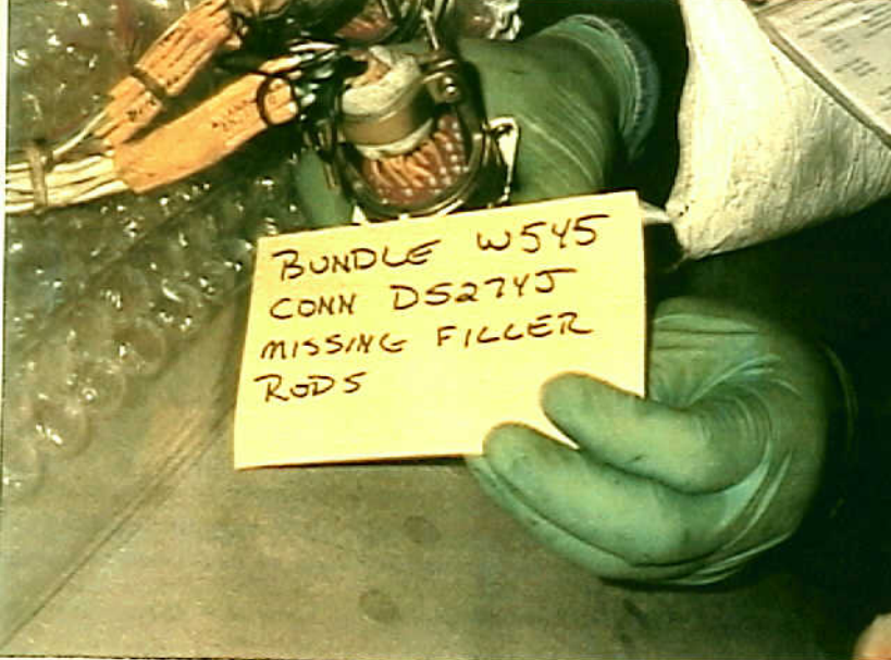
Systems 9 - 747-SL-20-048 - Fig. 19. Missing connector filler rods. The compromised environmental seal can contribute to internal connector corrosion.
