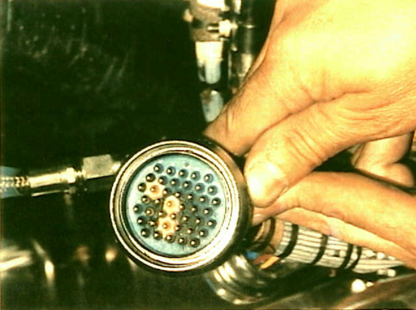
Systems 9 - 747-SL-20-048 - Fig. 15. Damage from hydraulic fluid on a connector grommet. Initially a color change is observed, then cracking occurs as the grommet dries out. If contamination is severe enough, all grommet material may be eroded.
