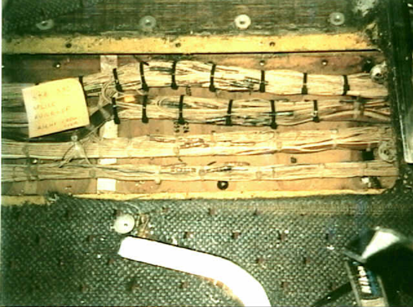
Systems 9 - 747-SL-20-048 - Fig. 13. Clumps created by concentrating a large number of splices on the flight deck floor crossover bundle. Splices should be staggered throughout the bundle, this reduces the potential for wire - to - wire (text cut-off).
