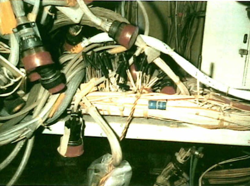
Systems 9 - 747-SL-20-048 - Fig. 12. Moisture resistant closed end splices correctly oriented up (Reference document, section 20-30-12). If they become oriented downward they can trap moisture, causing corrosion.
