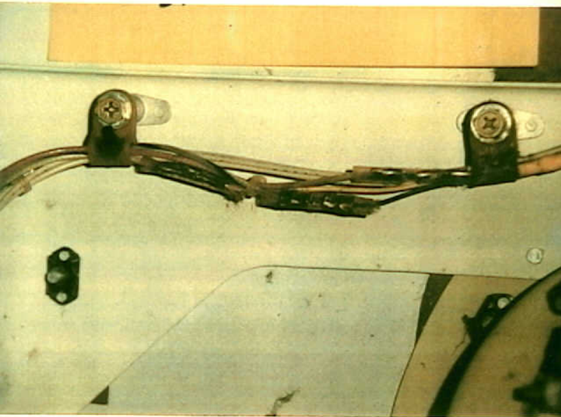
Systems 9 - 747-SL-20-048 - Fig. 11. General purpose splices used in the high moisture environment, of the aft cargo bay showing corrosion.
