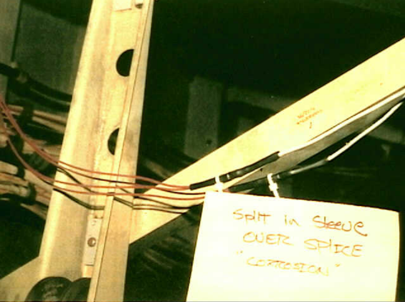
Systems 9 - 747-SL-20-048 - Fig. 10. Sleeving over splices failed, allowing splice corrosion.
