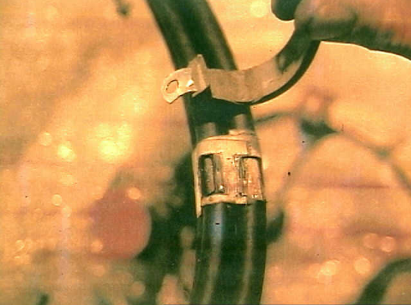
Systems 9 - 747-SL-20-048 - Fig. 1. Vibration caused chafing under the bundle clamp. Note that the clamp cushion shows little sign of wear.
