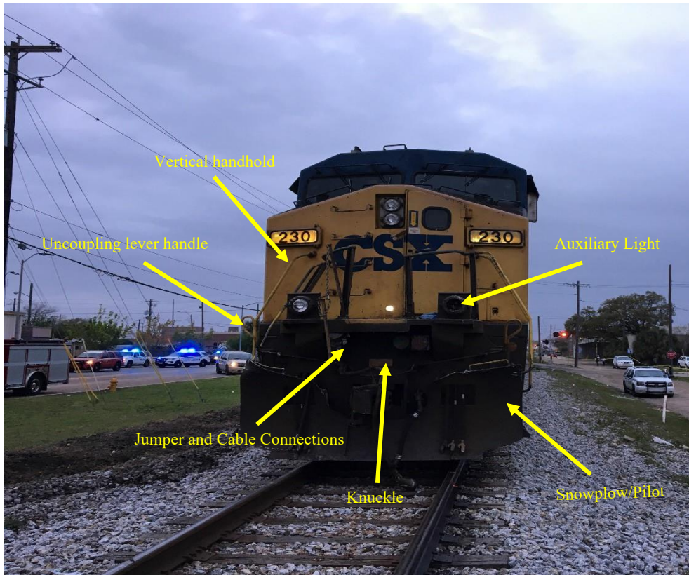
Photo #1: The lead locomotive showing the impact area and collision damage
