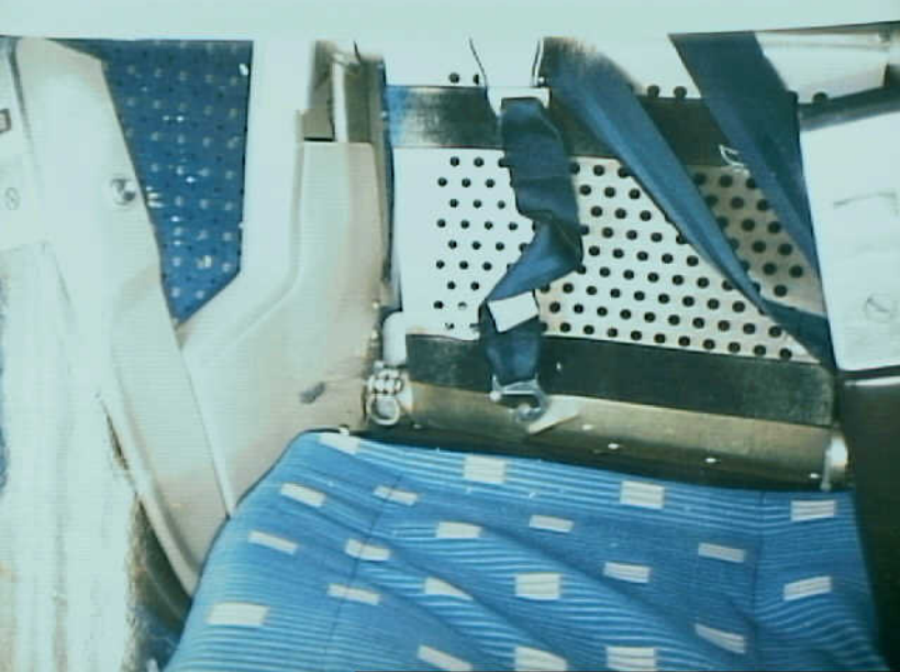
Survival Factors 6 - Photo 37. Interior damage, rows 12 and 13, looking forward.
