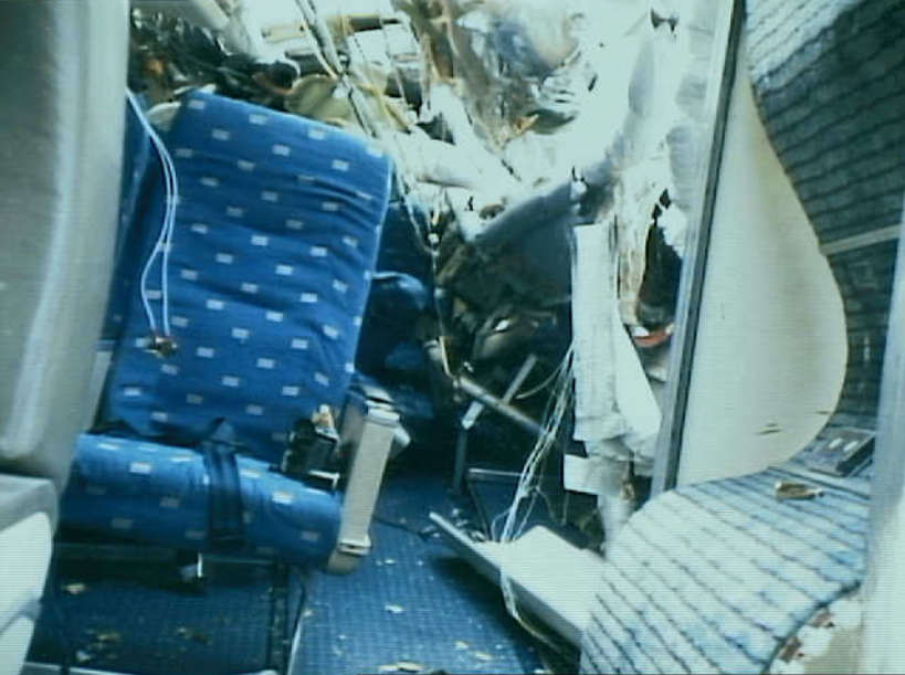
Survival Factors 6 - Photo 34. Interior damage, seat 8D, seat belt unattached.
