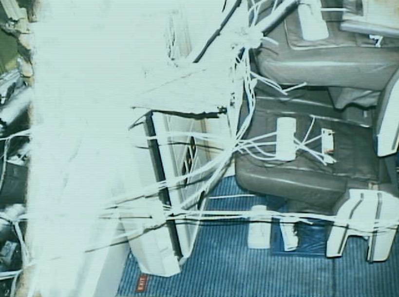
Survival Factors 6 - Photo 33. Interior damage, seat unit 4 EF, showing floor disruption.
