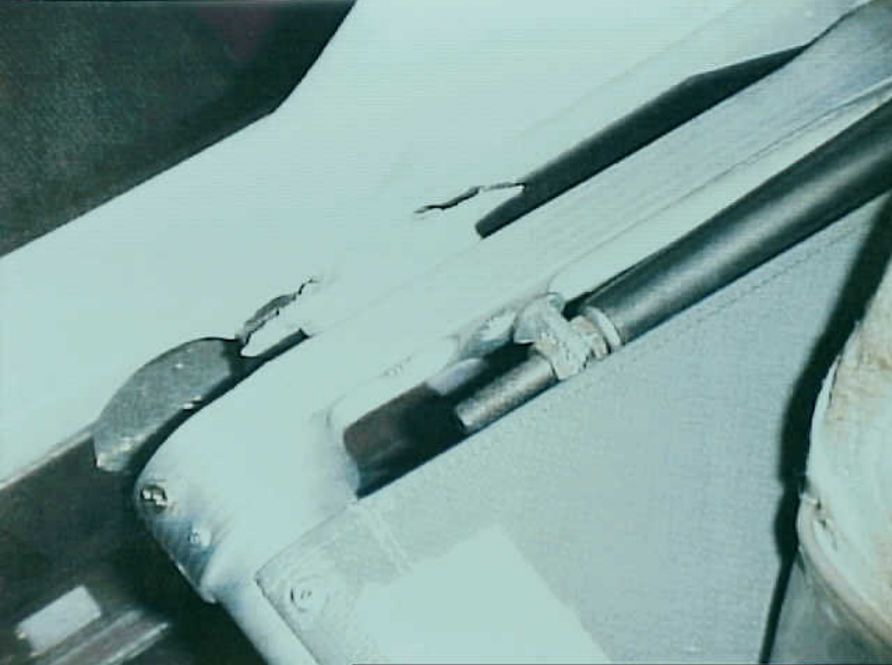
Survival Factors 6 - Photo 12. Inboard armrest attachment on seat ID.
