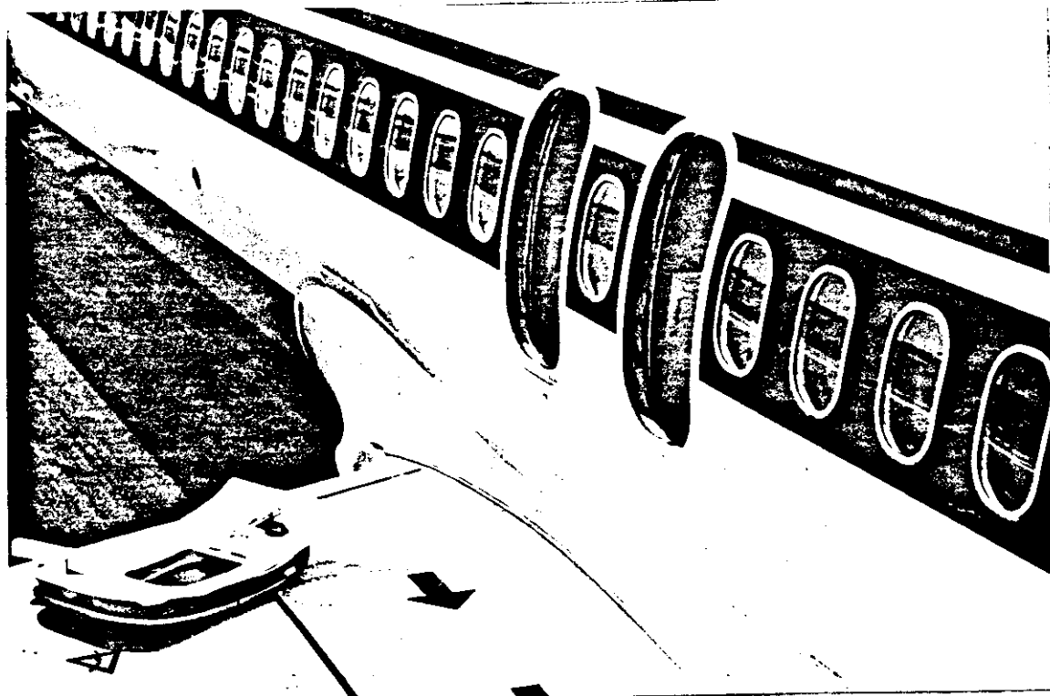
Photo. 2. Left side overwing emergency window exits, all 4 overwing exits were used.
