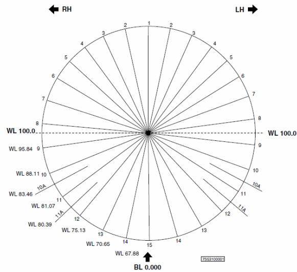
Figure 4 – SA-227AC Fuselage Stringer diagram
