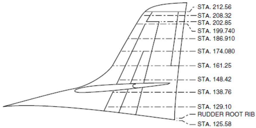
Figure 6 – SA-227AC Vertical Stabilizer and Rudder Station diagram
