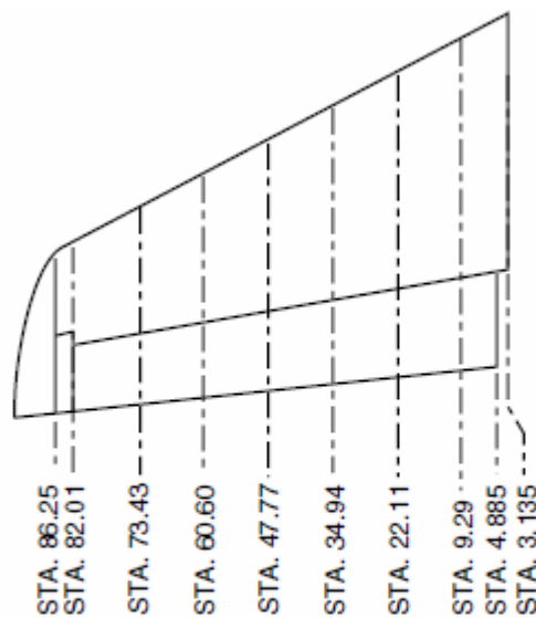
Figure 7 – SA-227AC Horizontal Stabilizer Station diagram
