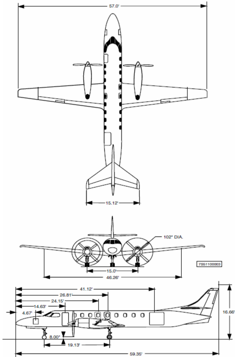
Figure 1 – Fairchild SA-227AC airplane
