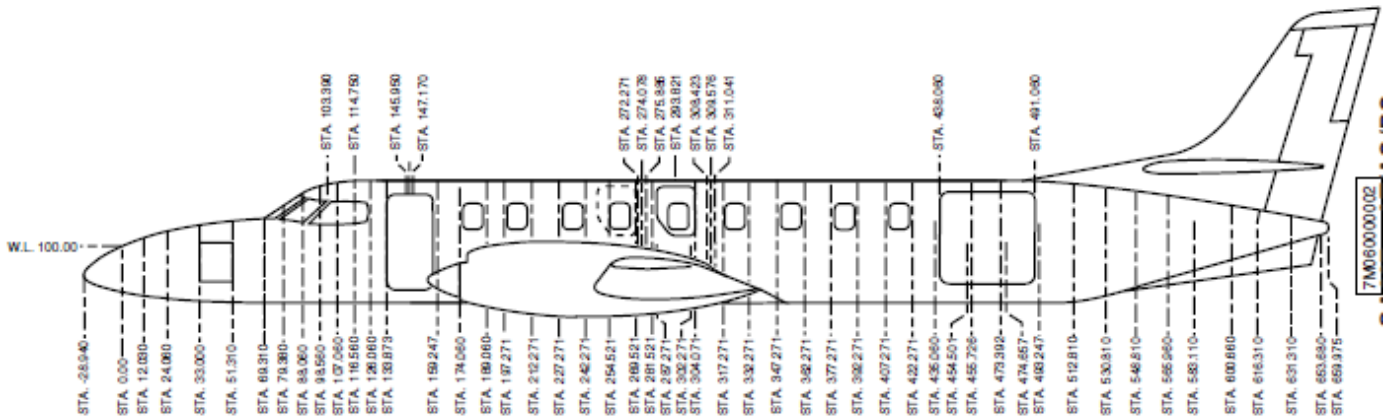
Figure 3 – SA-227AC Fuselage Station diagram
