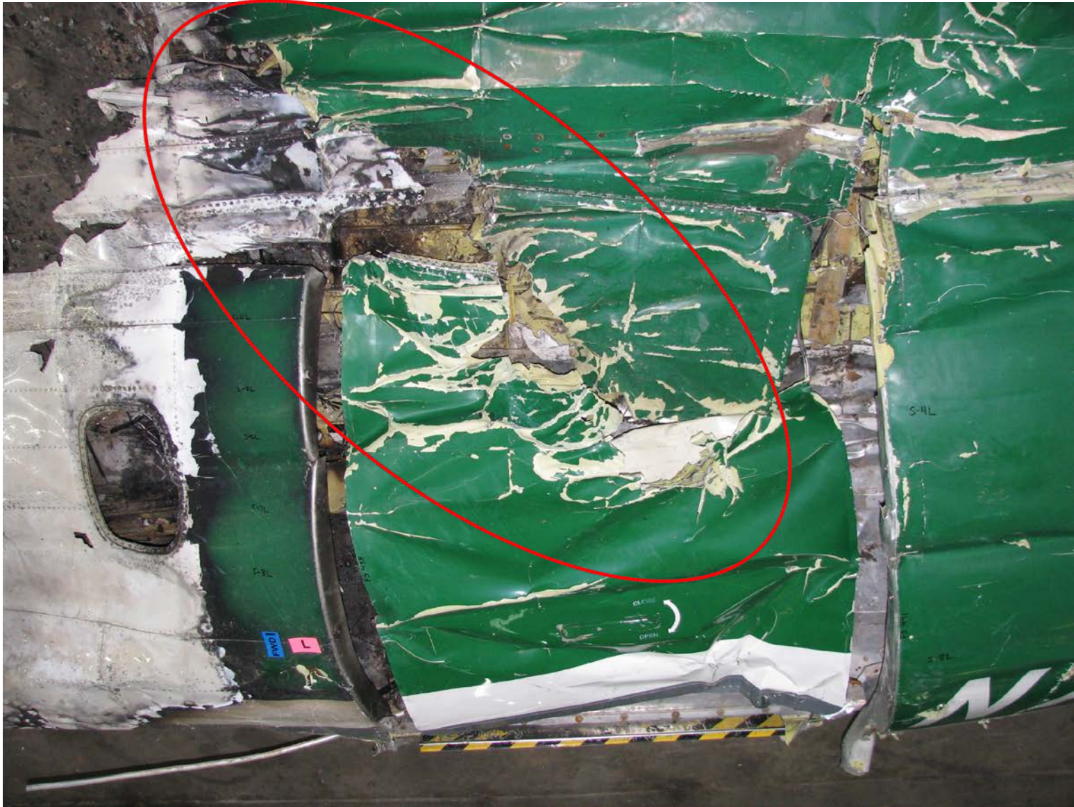
Figure 10 – Left fuselage damage
