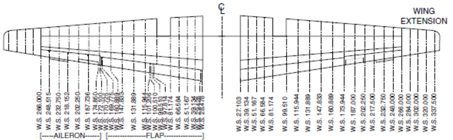
Figure 5 – SA-227AC Wing Station diagram
