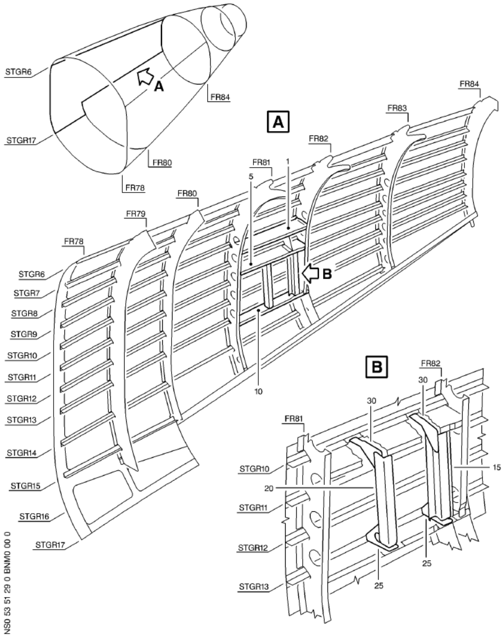
Side Shell RH,FR81-FR82, Stiffening Structure
