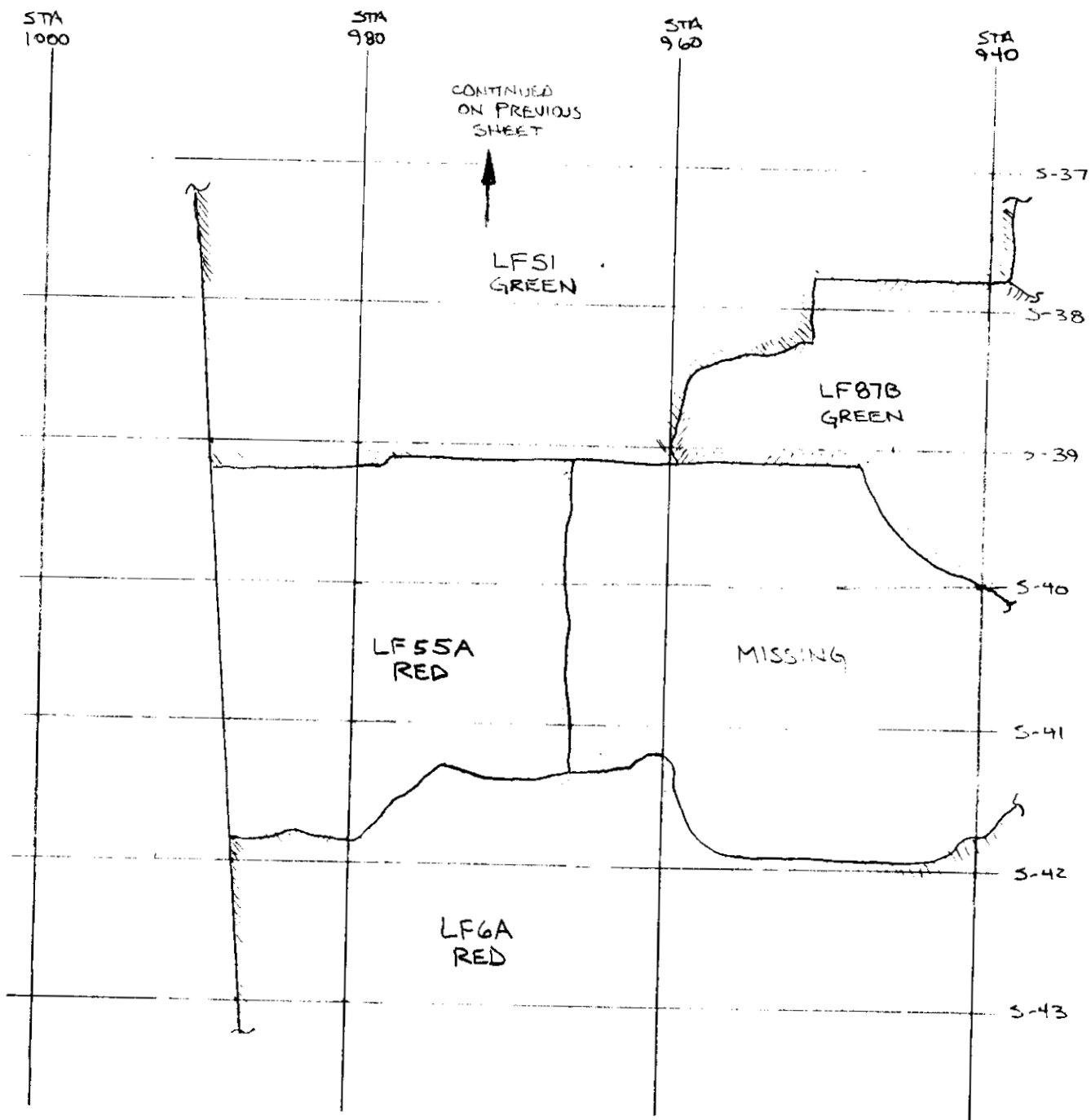
Left hand side fuselage skin Map (sheet 3 of 4)
