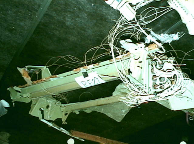
Structures 7 - RF-29 Photo 1
