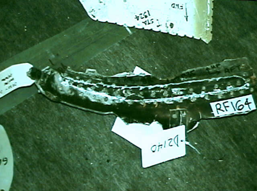
Structures 7 - RF-164 Photo 1
