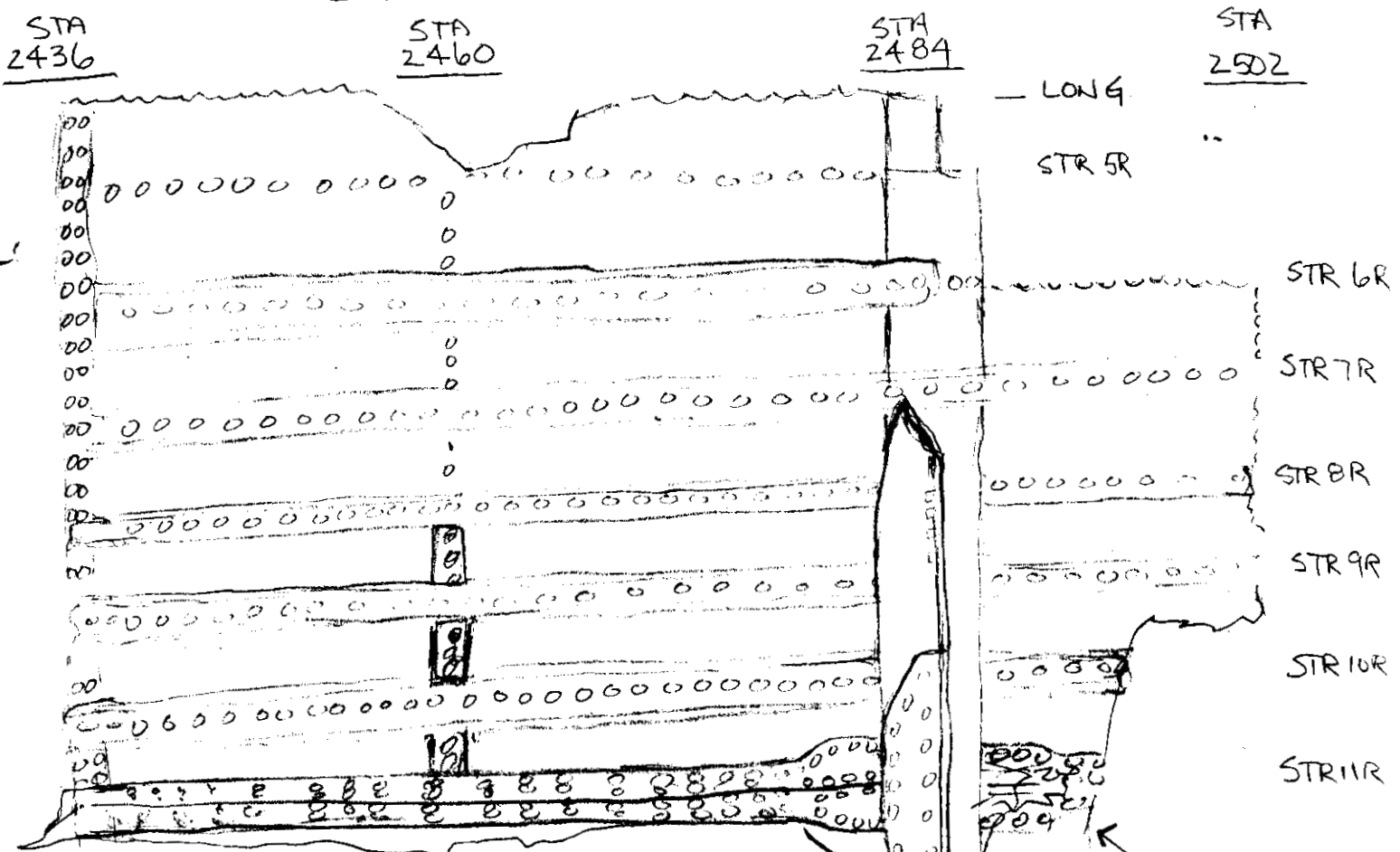
VIEW LOOKING OUTB'D
