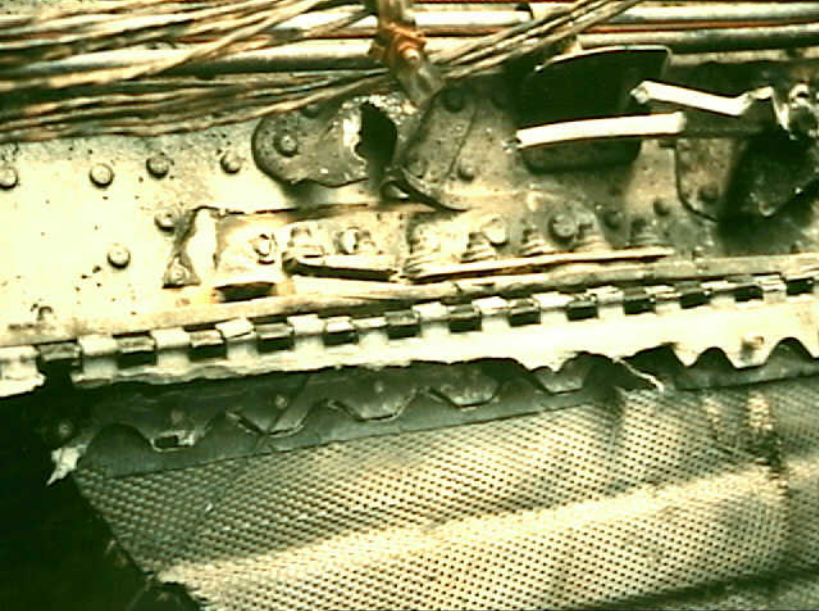
Structures 7 - Photo. 8 - View of the fractures flap hinge inboard side brace fitting.
