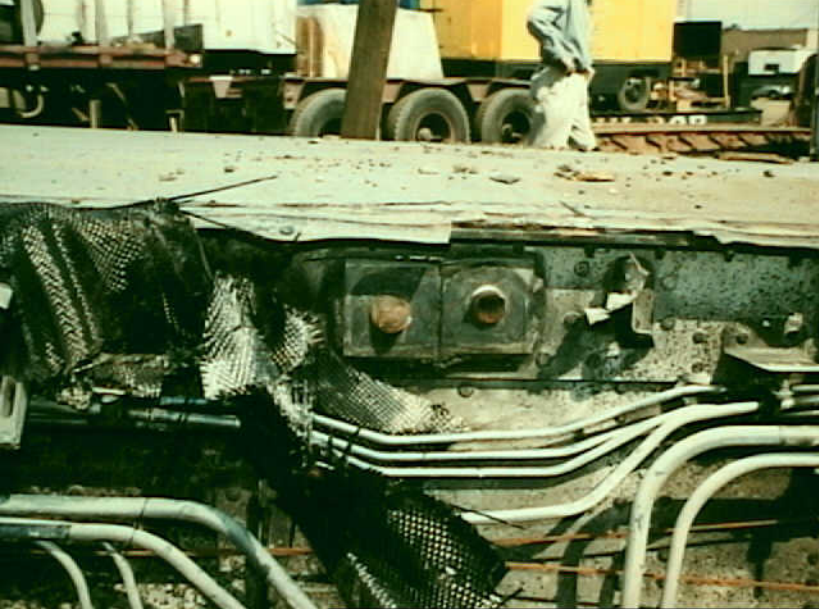
Structures 7 - Photo. 7 - View of the inboard attach fitting upper fasteners for the outboard flap hinge. Note the opposite direction of fractures.
