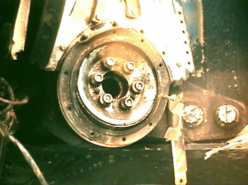
Structures 7 - Photo. 6 - View of inboard forward number 3 engine pylon attach fitting (tombstone fitting)
